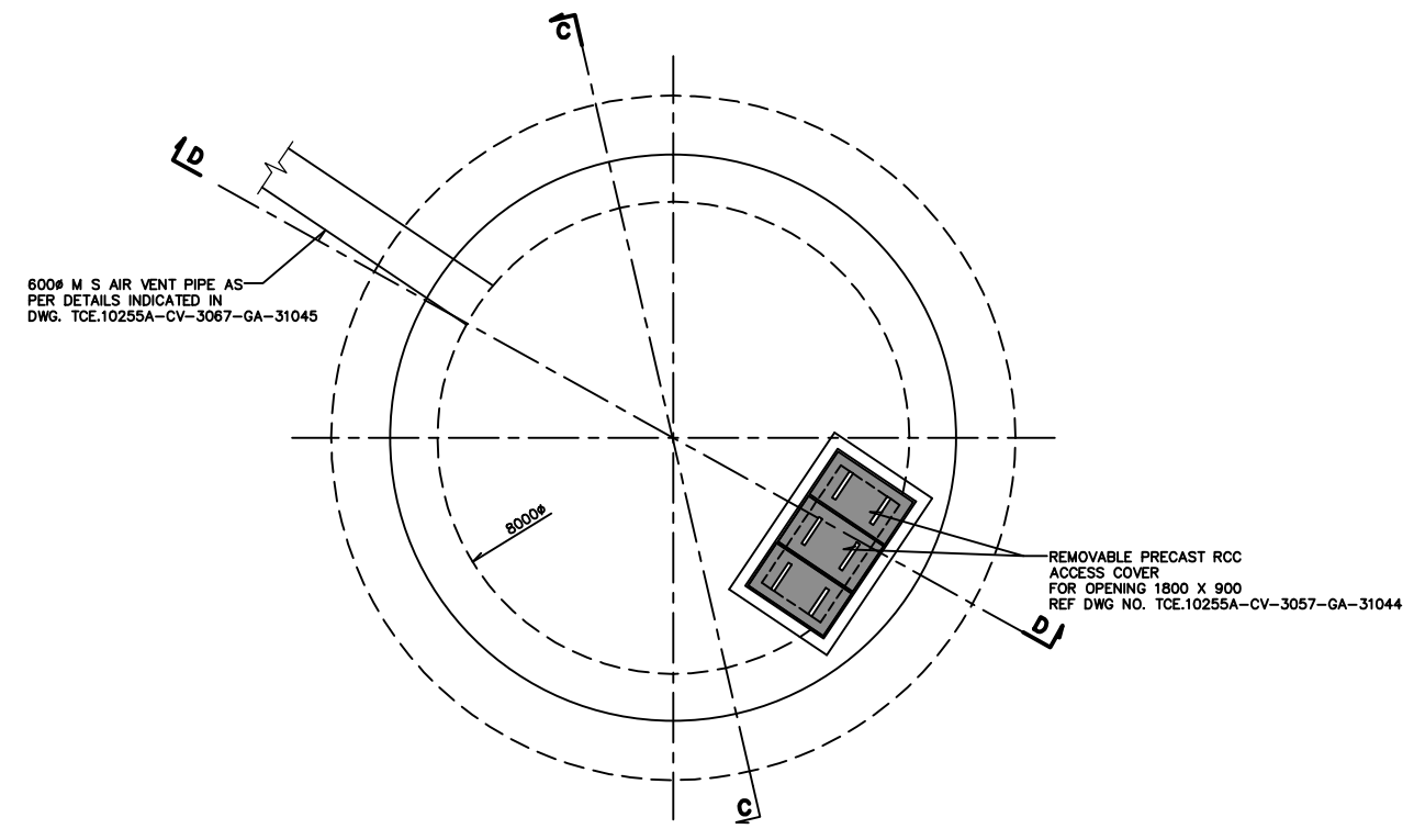
SECTIONAL PLAN A-A 1:50
