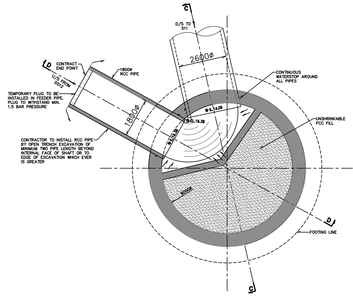
SECTIONAL PLAN B-B 1:50
